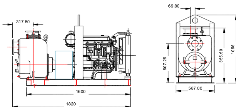
I-4 ALLPRIME Motor Diesel 38Cv
