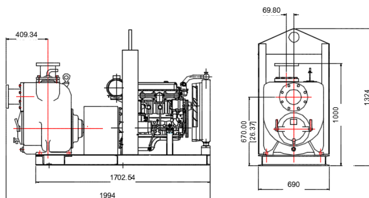
I-6 ALLPRIME Motor Diesel 82Cv
