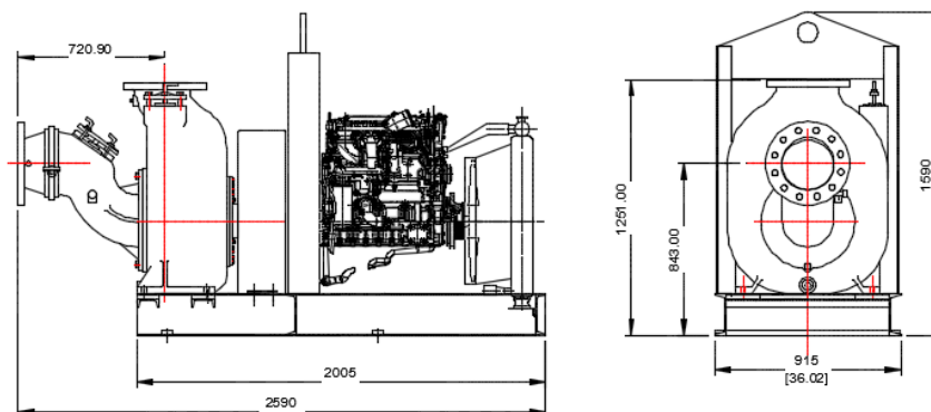
S-10ALLPRIME Motor Diesel 155Cv
